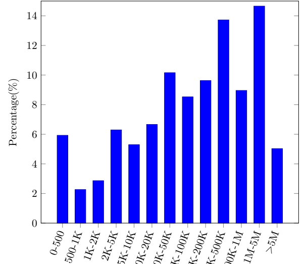
Fig. 5: Distribution of range lengths in the IP blacklist dataset.
