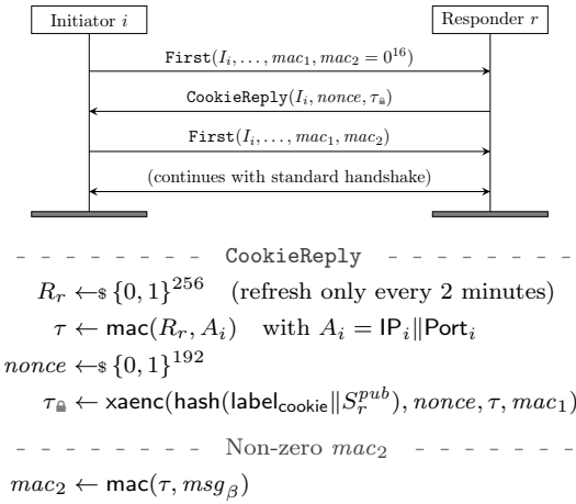
Figure 1c: Cookie mechanism under load.
