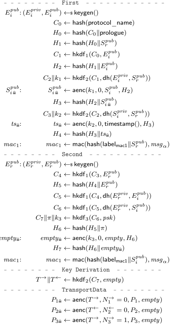
Figure 1b: Cryptographic Computations for Protocol Messages.
