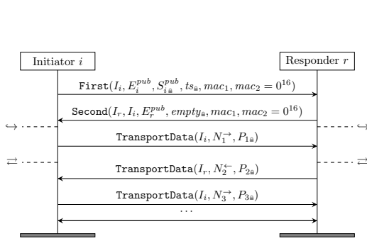
Figure 1a: WireGuard's protocol messages.
