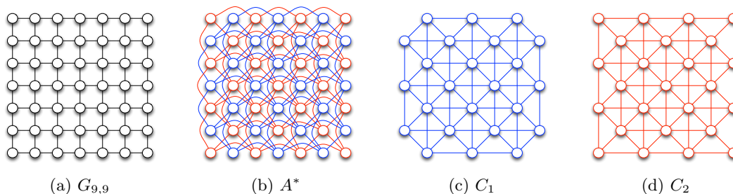
Figure 3: The grid G_{9,9} and the associated graph A^* .
