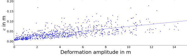
Figure 9: Sensitivity of e to the deformation amplitude for the L-shape. The point cloud represents the e all the samples of the testing data set. The regression line of equation y = 0.005716 \times x shows the low sensitivity of the U-Mesh to the deformation range.
