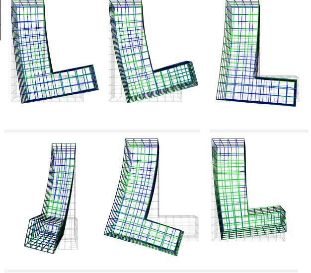
Figure 8: Samples of deformed L-shapes. In green is shown the reference solution, in blue the output of U-Mesh and in grey the rest shape.
