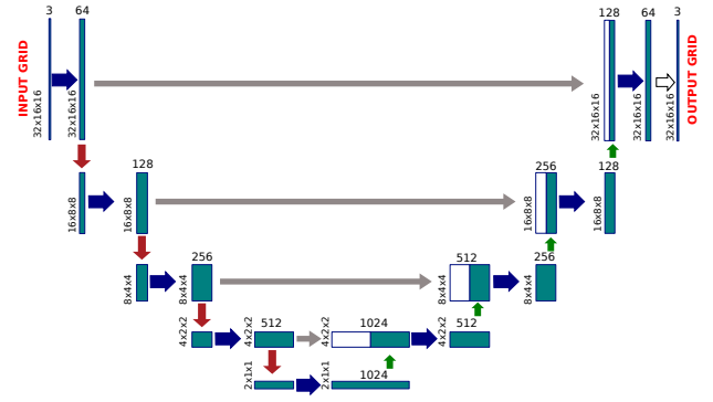
Figure 2: Network architecture for a beam with 28 \times 12 \times 12 nodes, padded to 32 \times 16 \times 16 , 64 channels in the first layer and 4 steps (see Fig. 1 for notations).
