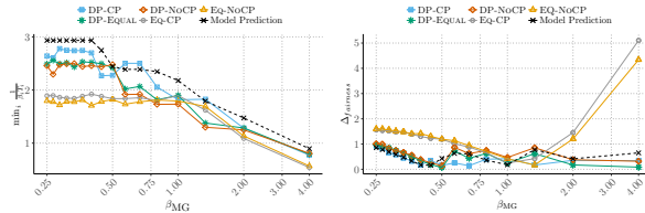
Fig. 14: Minimum throughput and \Delta_{fairness} for 2CG+MG.
