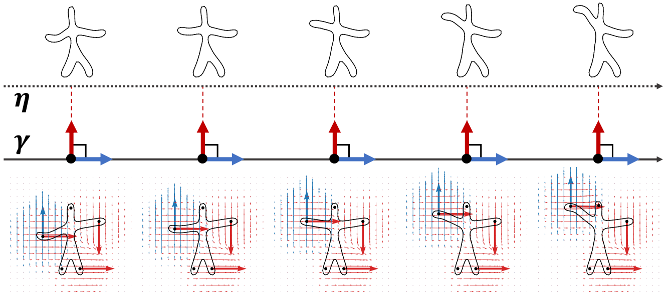
Fig. 2: [Bottom] . Illustration of a shape geodesic t \rightarrow \gamma(t) \star y_0 : the man-like shape (solid black contour) raises his left arm. This geodesic is parametrized by a single set of control points c_0 (black dots) and attached momentum vectors m_0 (bold blue arrows), to which corresponds the velocity field v_0 (light blue arrows). A second set of momentum vectors m (bold red arrows) attached to the same control points c_0 parametrizes the exp-parallelization of this shape geodesic. [Top] . Exp-parallel shape curve t \rightarrow \eta(t) \star y_0 to the shape geodesic \gamma \star y_0 : the exp-parallelization transfers the motion of the arm from one man (the one on the geodesic) to another one.
