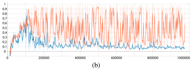
Figure 5: (a) Example of PPO getting trapped in a local minimum (top row) while PPO+SAUNA reaches a better optimum (bottom row). (b) \mathcal{V}^{ex} score for PPO (blue) and PPO+SAUNA (orange).
