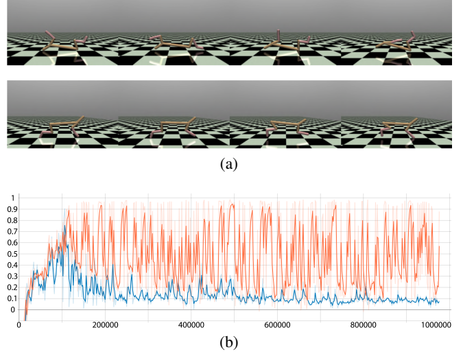
Figure 5: (a) Example of PPO getting trapped in a local minimum (top row) while PPO+SAUNA reaches a better optimum (bottom row). (b) \mathcal{V}^{ex} score for PPO (blue) and PPO+SAUNA (orange).
