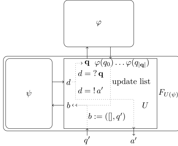
Figure 3: The universal used in the library.
