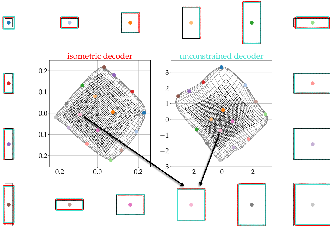
Figure 4. [Inner]. Latent spaces learned by the proposed mesh auto-encoder (left), and a modified architecture without norm scaling (right). For both, the black grid marks the encoded train rectangles, when the lighter grey grid marks the encoded test rectangles.
