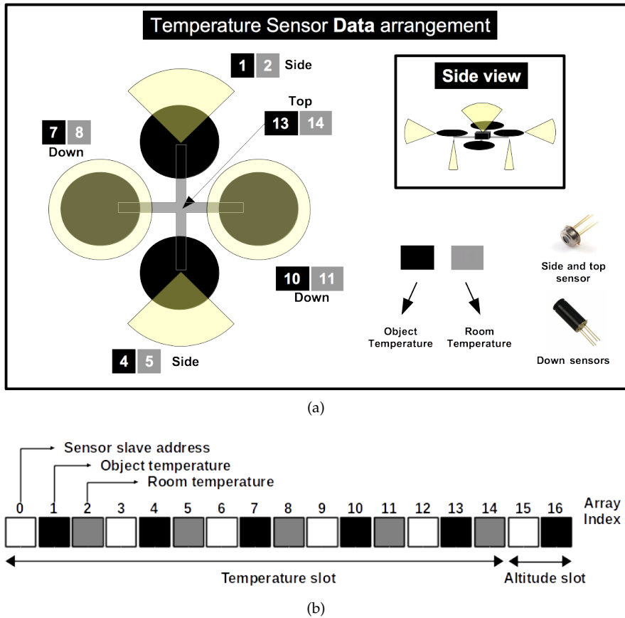
Figure 1. The MLX90614 sensors: (a) Sensor arrangement and identification number in the quad-rotor frame; (b) The message sent by the node for temperature is an array of floats, including all the measurements read by the Arduino board during a loop, i.e., temperature and sonar readings.
