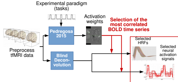
Fig. 2: Voxel selection procedure for the validation of the semi-blind deconvolution method on HCP data. The voxels are selected based on their correlation level with the EP.
