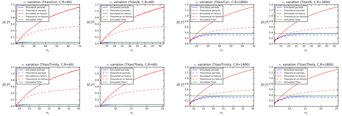
Figure 3: Evolution of overhead when \sigma_1 varies with C = R = 60s on the left and C = R = 1800s on the right.
