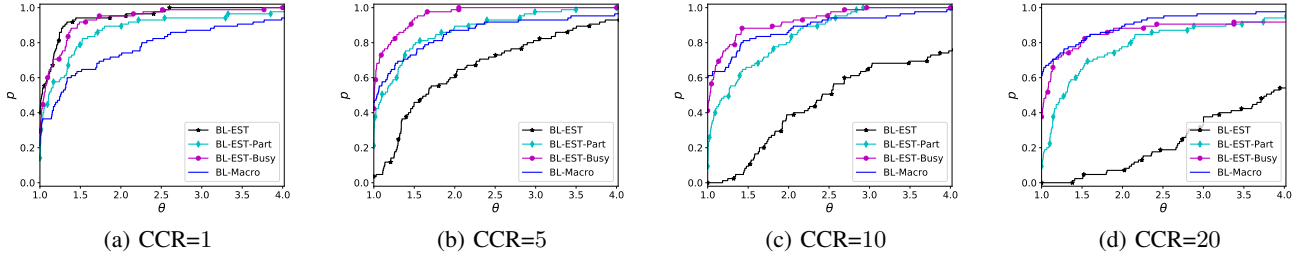
Figure 8: Performance profiles on big dataset, with CCR=\{1, 5, 10, 20\} .
