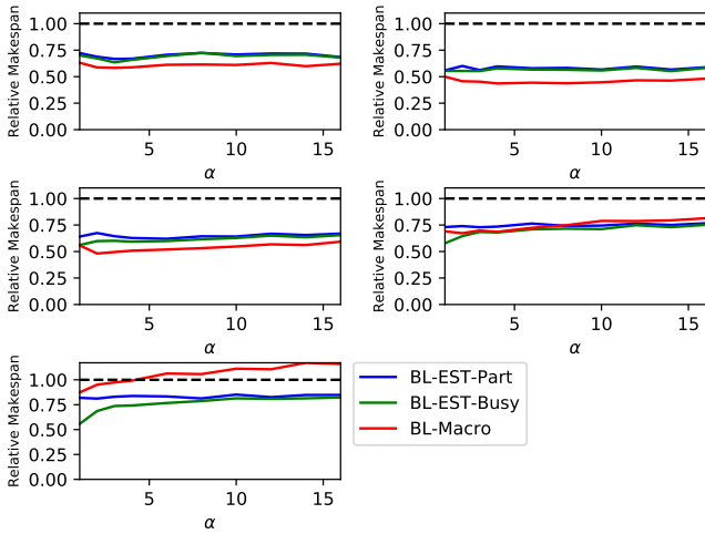
Figure 4: Relative makespan compared to BL-EST on the big dataset, as a function of the number of parts, with CCR=10 and with 2 (top left), 4 (top right), 8 (middle left), 16 (middle right), and 32 (bottom left) processors.
