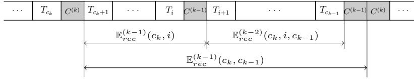
Figure 6: Placing checkpoints at level k - 1 : c_k and c_{k-1} are fixed, and we try possible locations i for an additional checkpoint between T_{c_k} and T_{c_{k-1}} . Again, all subproblems \mathbb{E}_{rec}^{(k-1)}(c_k, i) , with c_k \leq i < c_{k-1} , have already been computed, while \mathbb{E}_{rec}^{(k-2)}(c_k, i, c_{k-1}) is computed by the next level of dynamic programming level.
