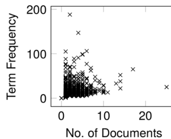
Fig. 1. Keyword statistics
