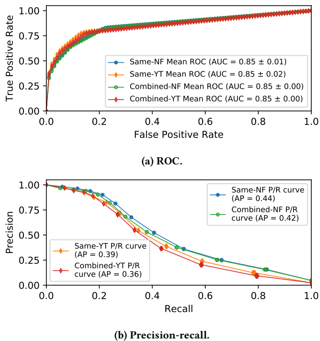
Figure 14: Inferring resolution switches, general model.
