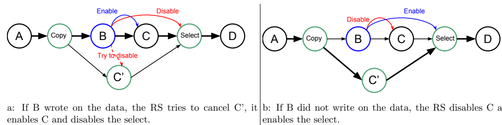
Figure 3 Graph of four tasks where B is an uncertain task and with speculation enabled. When B is over the RS update the next tasks, in (A) if B did write on the data, and in (B) otherwise.
