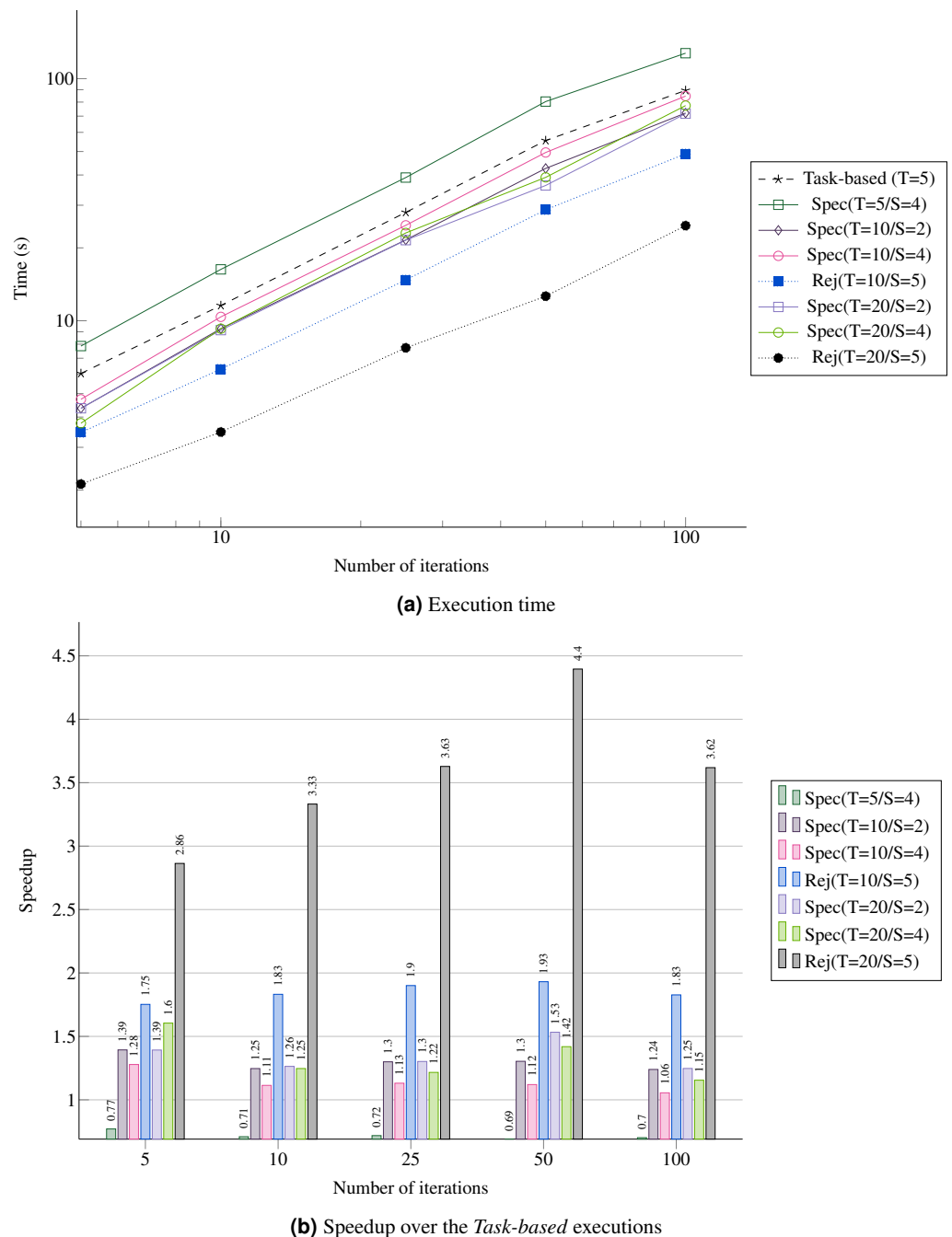
Figure 13 Performance for the REMC simulation with five replicas and five domains per replica. (A) Execution time; (B) Speedup over the Task-based executions.
