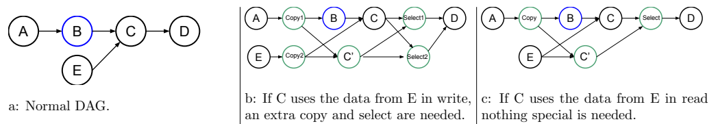
Figure 4 Graph of five tasks where B is an uncertain task and where C , the task use for speculation, uses data from another task E .
