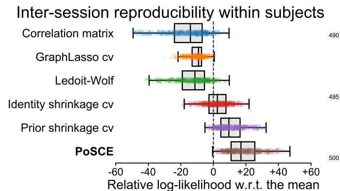
Figure 6: Fidelity to subject data. Boxplots represent the average log-likelihood of the data in a second session, which quantifies the relative similarities between respective sessions of 615 subjects from HCP. Shrinking the covariance towards population prior improves reproducibility compared with Pearson correlation, Ledoit-Wolf, and \ell_1 penalized estimators. PoSCE outperforms all other estimators.
