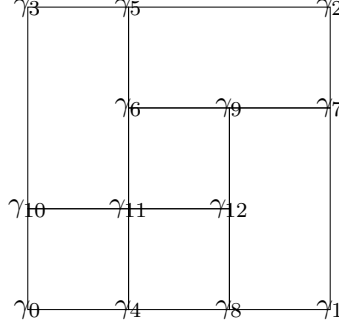
Figure 5: The T-mesh used in Example 7.3 to explicitly demonstrate how results from Section 3 can be used to find the dimension of \mathcal{S}_{\Delta \mathbf{m}, \mathbf{m}}^r .
