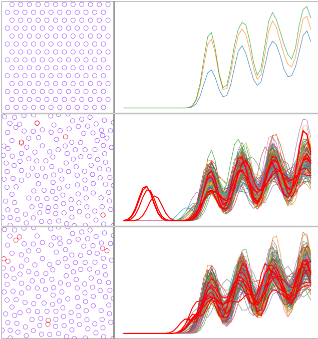
Figure 13: Failure case on a hexagonal grid: (top) exemplar input, (center) standard disk synthesis, and (bottom) synthesis with outlier removal. The pattern and distance between points are preserved locally but the global layout does not converge to a visually acceptable solution. Disks with the most outlying PCFs are colored in red at each stage. In the center left pattern, these correspond to several superimposed red disks, inducing the initial PCF bumps (center right).
