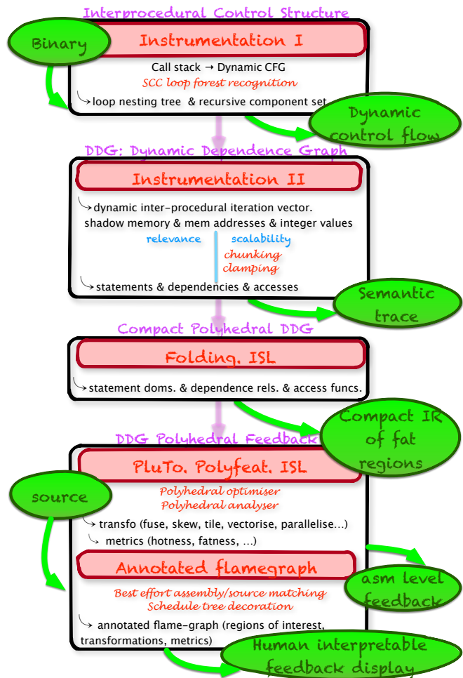
Figure 1. Overview over the POLY-PROF framework.
