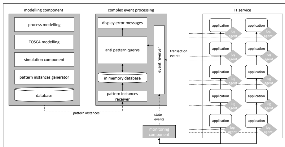
Fig. 7. Implementation architecture
