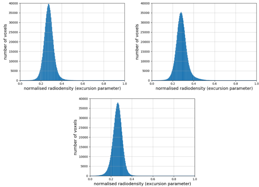
Fig. 5 Histograms of the normalized radiodensity distribution for core samples (clockwise - 1st, 2nd and 3rd cube).
