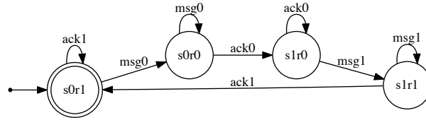
Fig. 9. Alternating bit protocol automaton
