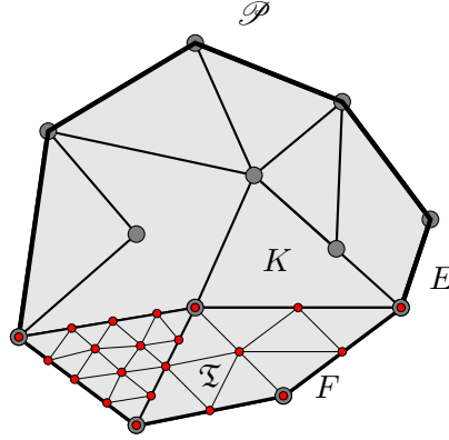
FIGURE 1. A domain partitioned with non-conforming polygonal elements K . Observe the sub-meshes discretising two different elements K with different granularity. The red dots represent the degrees of freedom associated with the sub-meshes and the gray dots with the mesh skeleton.
