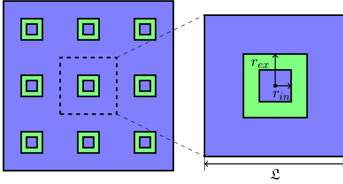
FIGURE 7. Sketch of the heterogeneous diffusive media with 3 \times 3 inclusions. Here r_{in} = \frac{1}{32} , r_{ex} = \frac{1}{16} , L = \frac{1}{3} , and the diffusive coefficient is \kappa = 1 (blue) and \kappa = 10^5 (green).
