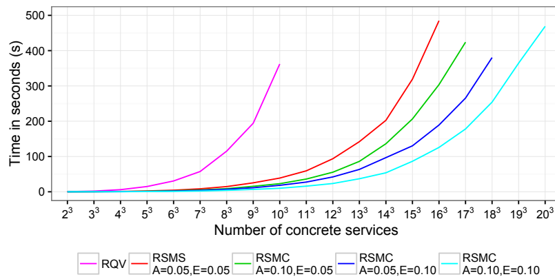
Figure 3 Adaptation time for RQV versus RSMC
