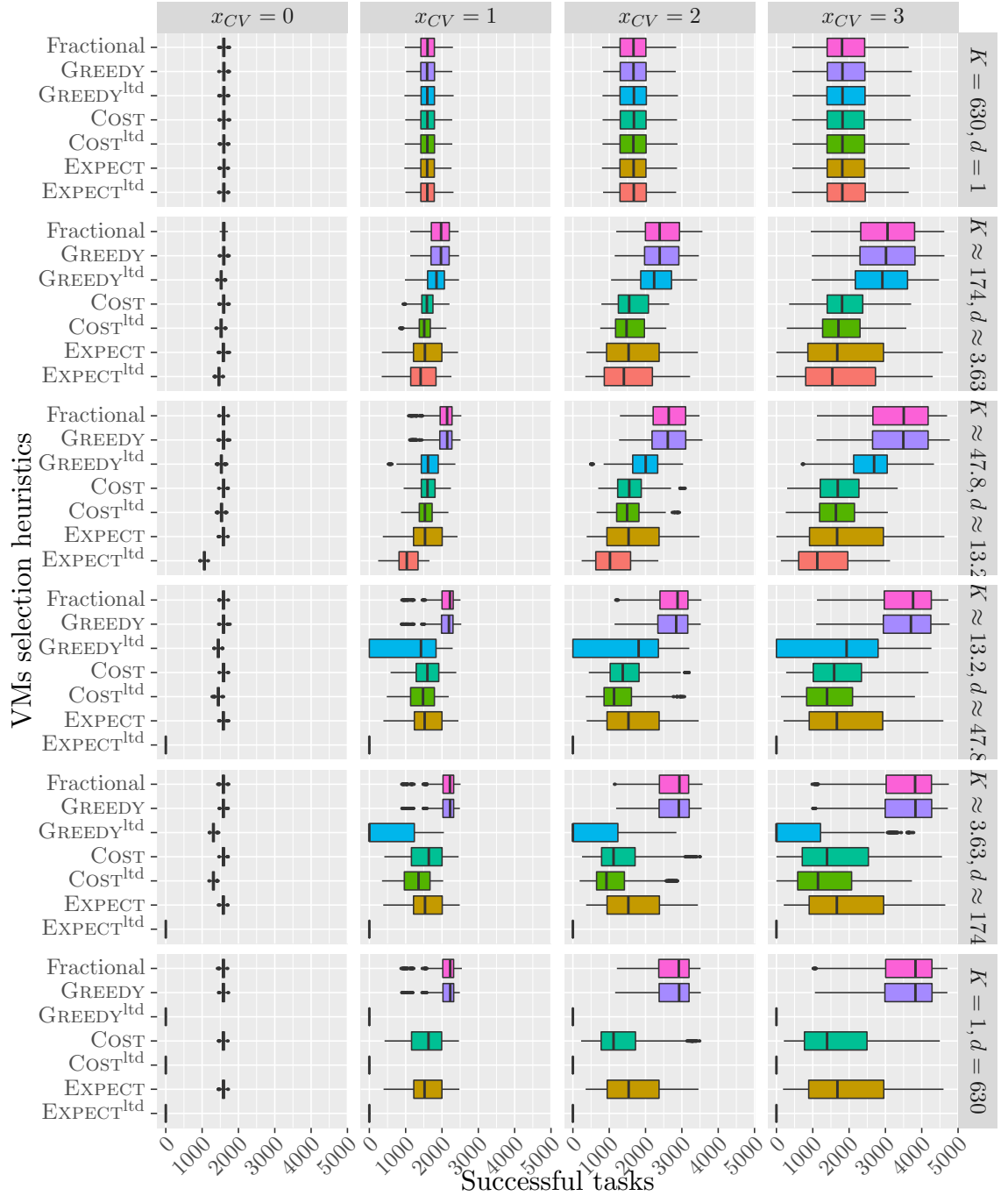
Figure 6: Number of successfully executed tasks of different methods to choose VMs when interrupting tasks with heuristic OPTRATIO. Each of the 100 platforms is generated with m_j = 10 , M = 60 , c_j = s_j and is used 10 times with b = 630 . The values for d and K follows a geometric progression between 1 and 630. Execution times follow either a lognormal distribution with x_{CV} = 0, 1, 2, 3 .
