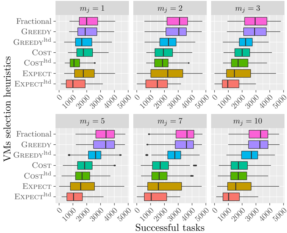
Figure 4: Number of successfully executed tasks of different methods to choose VMs when interrupting tasks with heuristic OPTRATIO. Each of the 100 platforms is generated with m_j = 1, 2, 3, 5, 7, 10 , M = 60 and is used 10 times with b = 630 and d \approx 13.2 ( K \approx 47.8 ). Execution times follow lognormal distributions with x_{CV} = 3 .
