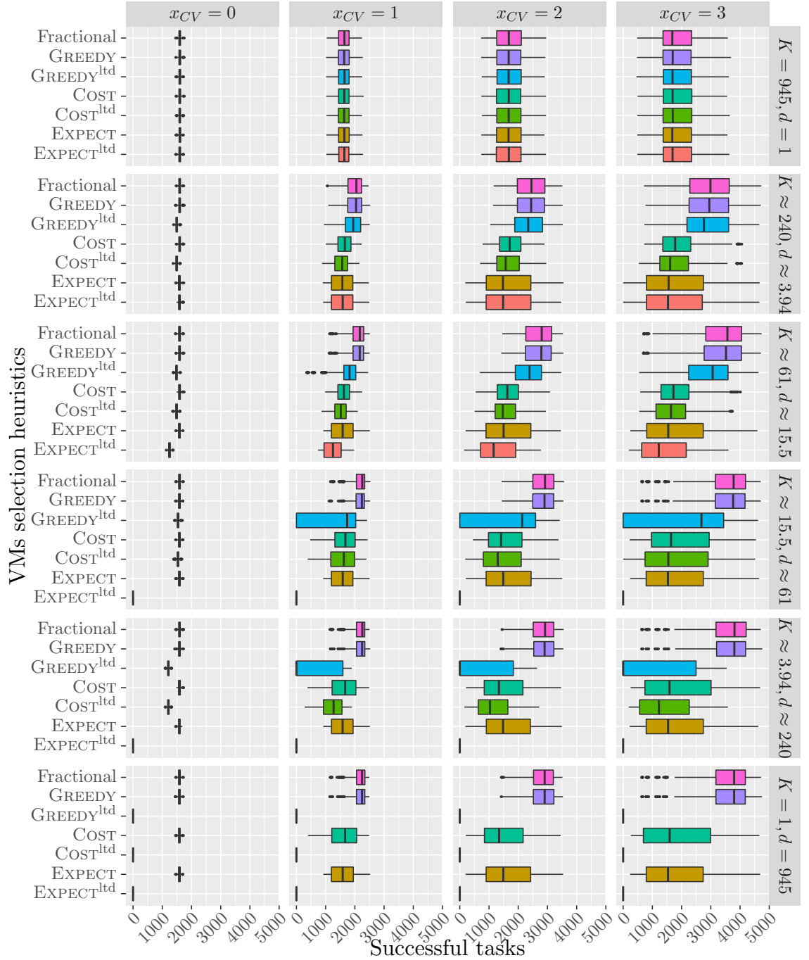
Figure 7: Number of successfully executed tasks of different methods to choose VMs when interrupting tasks with heuristic OPT-RATIO. Each of the 100 platforms is generated with m_j = 10 , M = 60 , c_j = 1.5s_j and is used 10 times with b = 945 . The values for d and K follows a geometric progression between 1 and 945. Execution times follow either a lognormal distribution with x_{CV} = 0, 1, 2, 3 .
