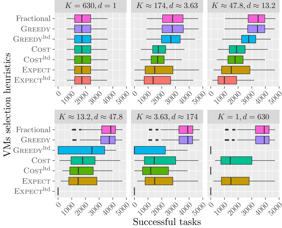
Figure 3: Number of successfully executed tasks of different methods to choose VMs when interrupting tasks with heuristic OPTRATIO. Each of the 100 platforms is generated with m_j = 10 , M = 60 and is used 10 times with b = 630 . The values for d and K follows a geometric progression between 1 and 630. Execution times follow either a lognormal distribution with x_{CV} = 3 .
