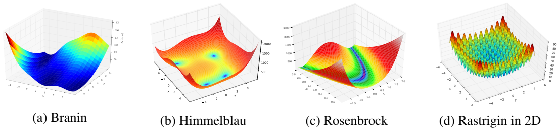
Figure 1: Benchmark functions 5
