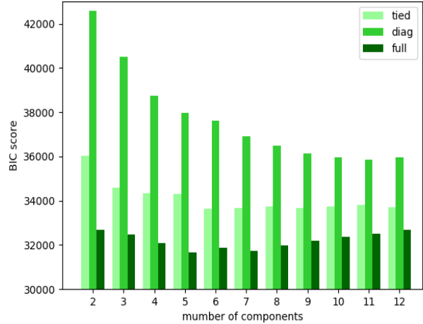
Figure 2: BIC scores of Gaussian mixture models with various types of covariance matrix and numbers of components
