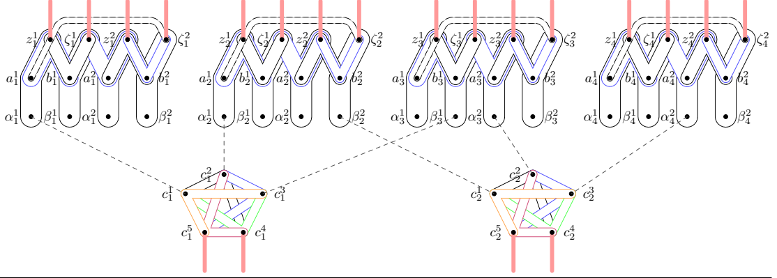
Figure 3 An example of the reduction for \Phi = (x_1 \vee x_2 \vee \bar{x}_3) \wedge (\bar{x}_2 \vee x_3 \vee x_4) . The dotted lines join two vertices that are identified. The thick red lines indicate the handicap vertices.
