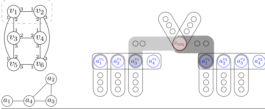
Figure 4 Illustration of the case 1 from the proof of Theorem 8, with a cubic graph \Gamma (top left, with an ordering on the neighbours of each vertex), F a graph on four vertices (bottom left), and k = 3 . We have \delta(F) = 1, d(a_1) = 1, d(a_2) = d(a_3) = 2 , and d(a_4) = 3 = \Delta(F) . Moreover \gamma = 2, \beta = 1, \gamma_1 = \gamma_2 = \gamma_3 = 1 . To the right, a part of the hypergraph which corresponds to the subgraph of \Gamma in the dashed box: two hyperedges for v_1, v_2 with blue vertices, two dashed hyperedges for edge v_1v_2 = e_3(v_1)e_1(v_2) and leaves with new vertices (unlabeled vertices).
