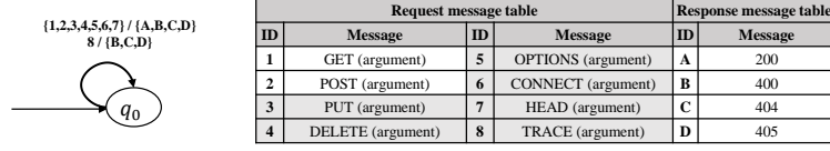
Fig. 5: Inferred HTTP state machine
