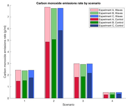
(b) Carbon monoxide emissions rate.
