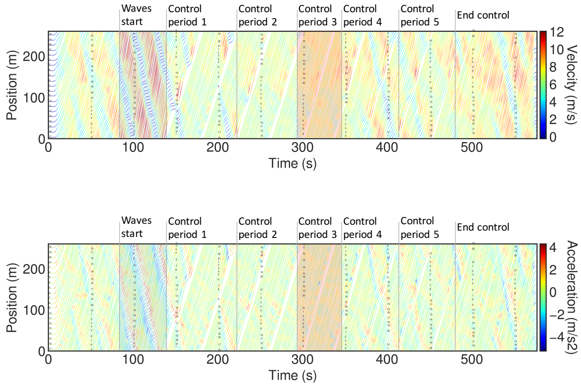
Figure 2: Vehicle trajectories for all vehicles in Experiment A color coded by, velocity (top), and acceleration (bottom). The time under which traffic waves are present is shaded blue, while the control period used for analysis, where the AV is actively dampening traffic waves is shaded red.
