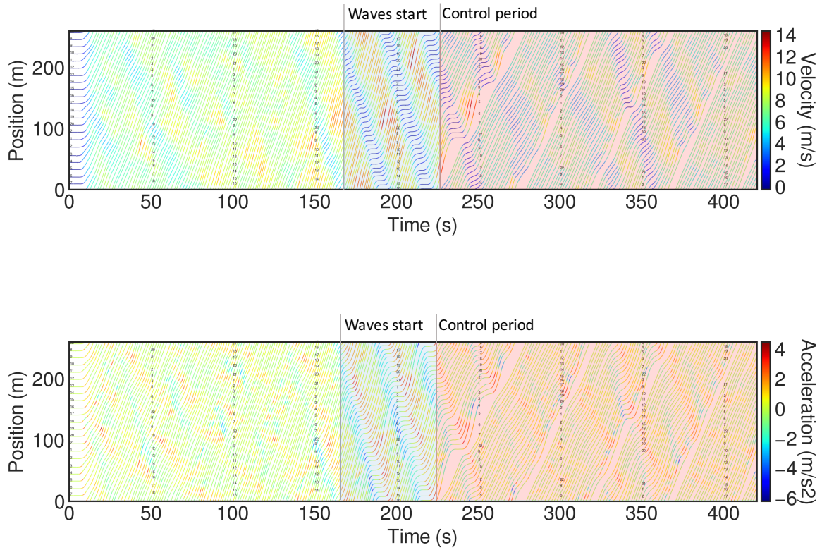
Figure 4: Vehicle trajectories for all vehicles in Experiment C color coded by, velocity (top), and acceleration (bottom). The time under which traffic waves are present is shaded blue, while the control period used for analysis, where the AV is actively dampening traffic waves is shaded red.
