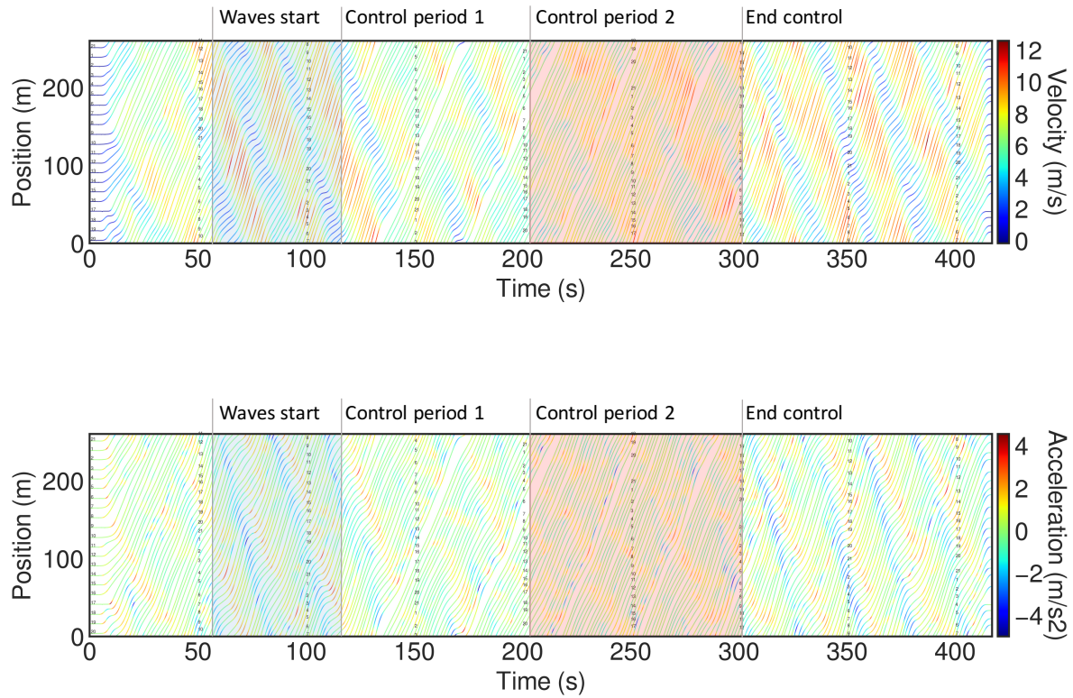
Figure 3: Vehicle trajectories for all vehicles in Experiment B color coded by, velocity (top), and acceleration (bottom). The time under which traffic waves are present is shaded blue, while the control period used for analysis, where the AV is actively dampening traffic waves is shaded red.
