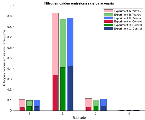
(c) Nitrogen oxides emissions rate.
