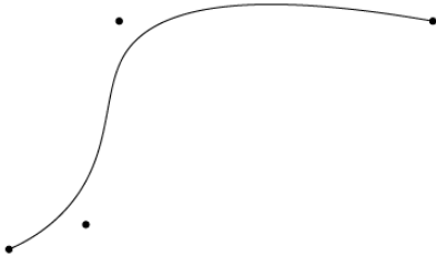
Figure 10: A planar B-Spline and its control points.
