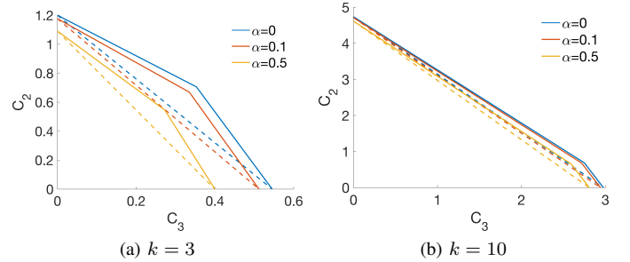
Fig. 8: Capacity region for a system of buffer size one and varying number of links k , decoherence rates \alpha , and entanglement generation rate \mu = 1 . The solid lines are the upper boundaries of the capacity region, and the dashed are TDM lines.
