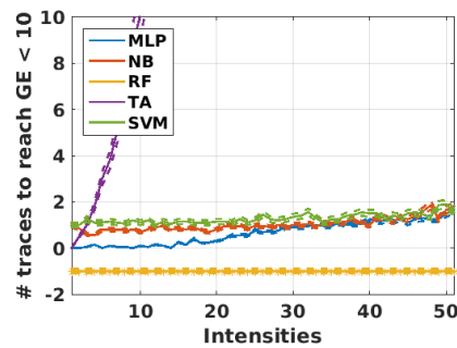
(f) DPAv4, value model, guessing entropy
