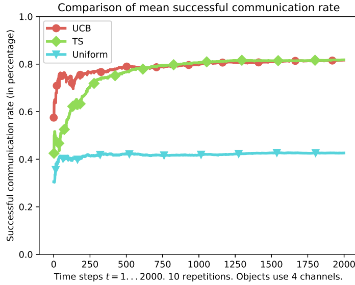
Fig. 4: Less than 400 communication slots ( i.e. , less than 100 trials in each channel) suffice for the two learning objects to reach a successful communication rate close to 80%, which is twice as much as the non-learning (uniform) object, which stays around 40% of success. Similar gains of performance were obtained in many different scenarios.
