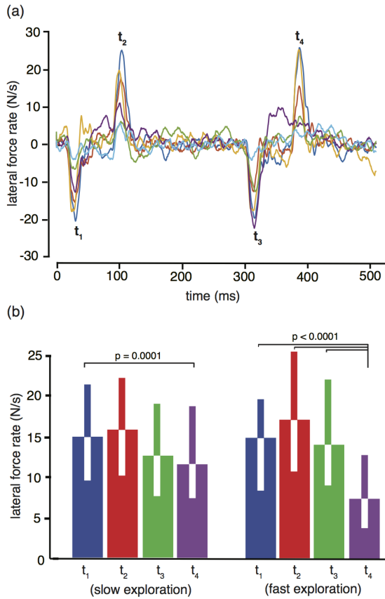
Fig. 6. (a) One example per participant chosen from the slow exploration of consecutive ultrasonic square signals of 70 ms duration. t_1, t_2, t_3 and t_4 represent the four peak changes in the lateral force induced by the ultrasonic step transitions. (b) For each of the four transitions, the peak rate of change of the lateral force was computed across all the trials of the experiment (Median \pm IQR). The computation was respectively performed for the slow exploration (left) and the fast exploration (right).
