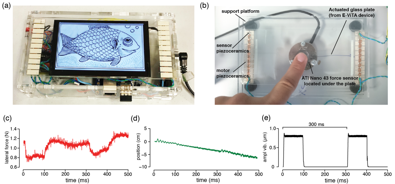
Fig. 1. (a) The visuo-haptic ultrasonic device E-ViTa, which was used to deliver ultrasonic square stimulations in the psychophysical experiments. (b) The glass plate from the E-ViTa device was mounted on a force transducer based on a 3-axis ATI Nano43 force sensor (c) In experiment 3, the recording of the amplitude of ultrasonic vibration and of the interfacial forces enabled the analysis of the precise contact mechanics induced by the ultrasonic signals. (d) The center of pressure of the fingertip hence the speed of exploration could be computed out of the forces and torques recorded in experiment 3. (e) In all three experiments, two consecutive identical square ultrasonic pulses were delivered when the finger reached the middle of the glass plate.
