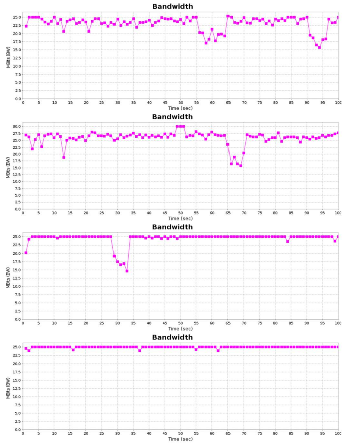
Fig. 10 Maximum throughput measurements
