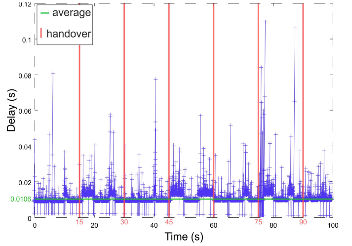
Fig. 9 Quake3 in the proposed solution
