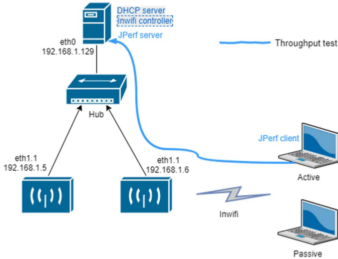
Fig. 6 Testbed
