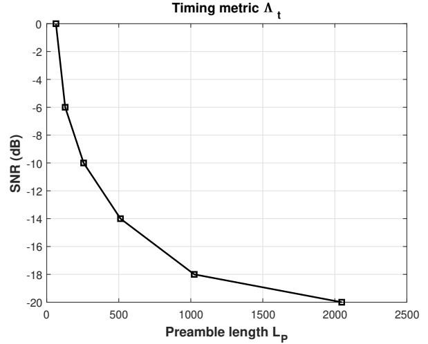
Figure 9. Evolution of the SNR threshold.
