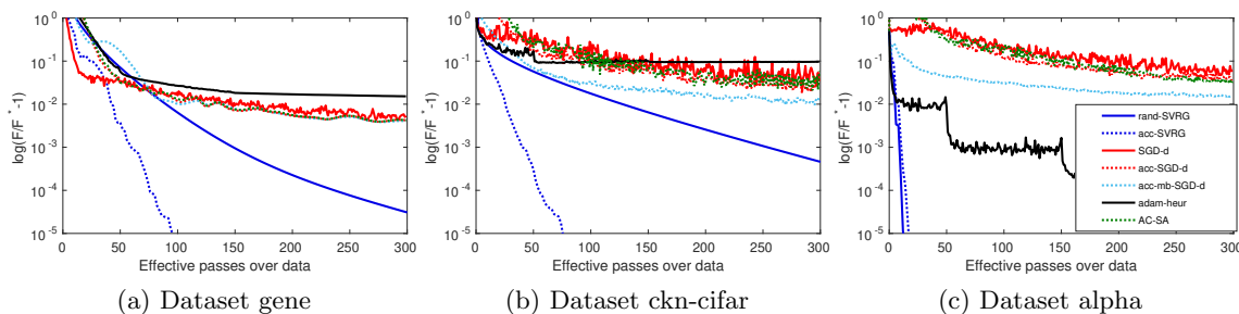
Figure 2: Same experiment as in Figure 1 with \lambda = 1/100n .
