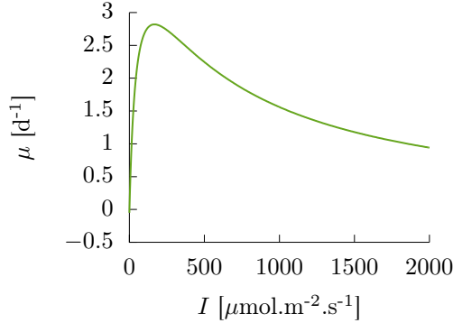
Figure 2: Growth rate (26) for the steady states to (20).
