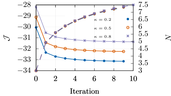
Figure 5: Evolution of the cost function \mathcal{J} in (78) (solid lines) and of the parameter N (dashed lines) with respect to the iteration for different homogeneous initial conditions.
