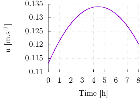
Figure 3: Velocity found when allowing a deviation of 5 % with respect to the optimal productivity for an initial condition C_i^0 = 0.3 .
