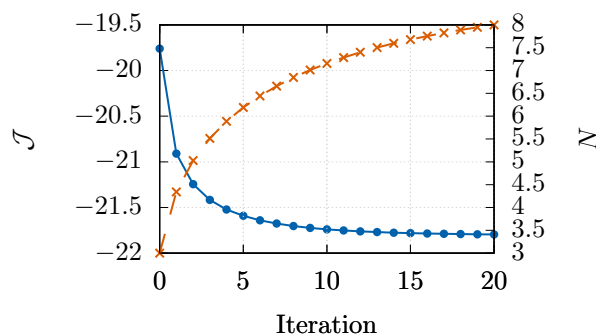
Figure 7: Evolution of the cost function \mathcal{J} in (78) (solid line) and of the parameter N (dashed line) with respect to the iteration for non-homogeneous initial conditions for the biomass density given in (92) and (93) and the photoinhibition rate given in (94) and (95).
