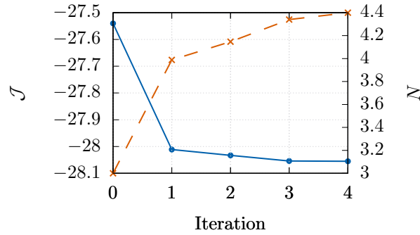
Figure 6: Evolution of the cost function \mathcal{J} in (78) (solid line) and of the parameter N (dashed line) with respect to the iteration for homogeneous initial conditions when optimizing only N for a velocity equal to 0.001 \text{ m}\cdot\text{s}^{-1} .
