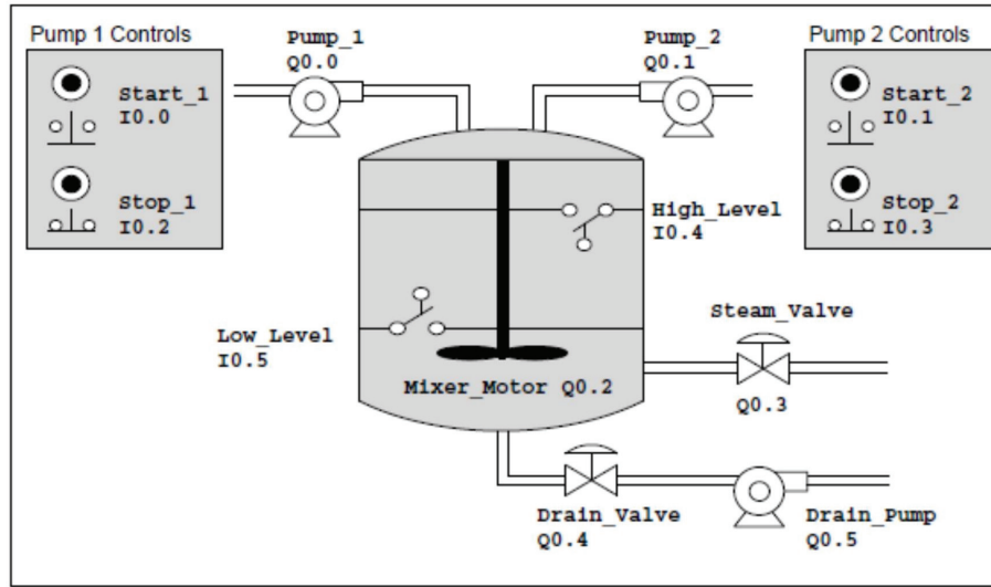
Figure 3. Input/output connections for the liquid mixing control system [11].
