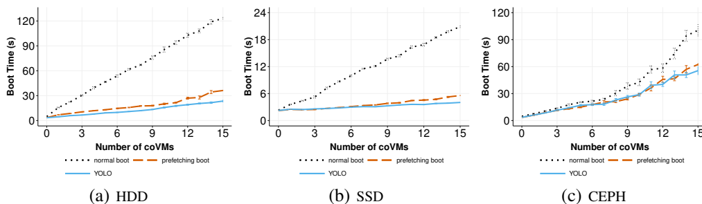
Fig. 12: Boot time of 1 VM (with shared image disk, write through cache mode ) under I/O contention environment
