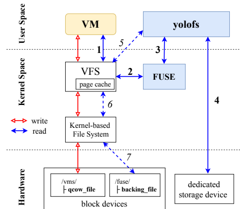
Fig. 7: yolo fs read/write data flow
