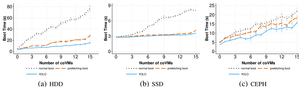
Fig. 13: Boot time of 1 VM (with shared image disk, write through cache mode ) under memory usage contention environment
