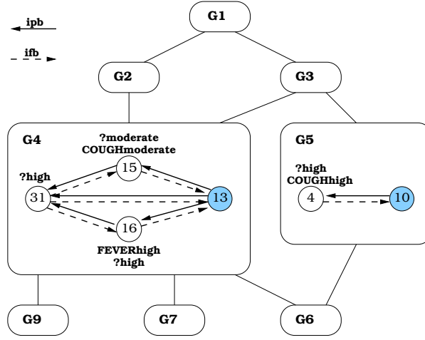
Fig. 6. Hierarchy of concept graphs about medical histories with inverse relation ifb . Only concept graphs whose concepts have their support greater than one are shown.
