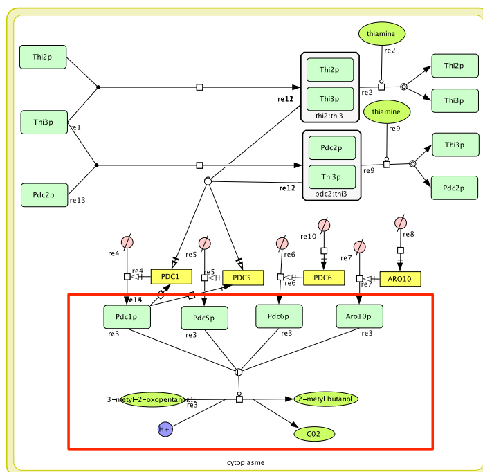
Figure 14: Explicit model of the 3-methyl-2-oxopentanoate decarboxylase system, outlining in red the part of the model considered when performing hierarchical modeling
