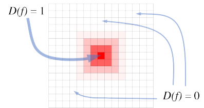
Figure 9: Example of propagation of the D(f) values on the domain boundary, with k = 4 .
